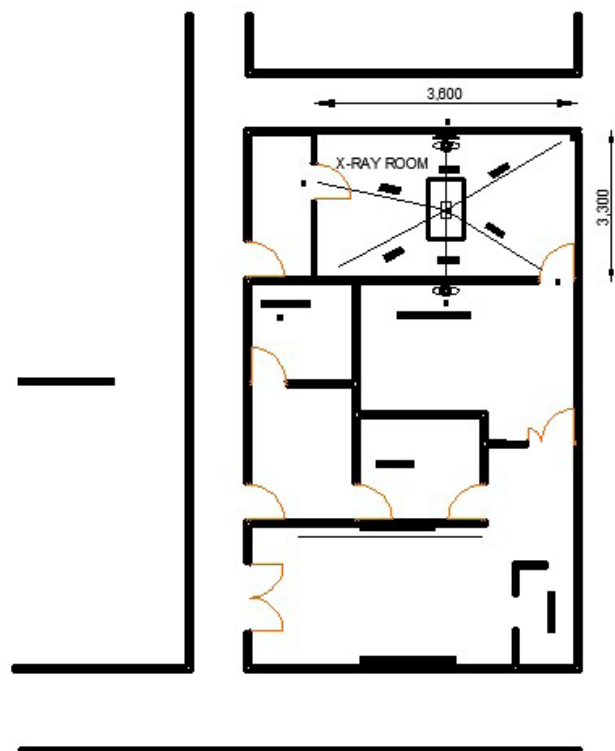
Figure 2. X-ray Room Layout for Center Y
